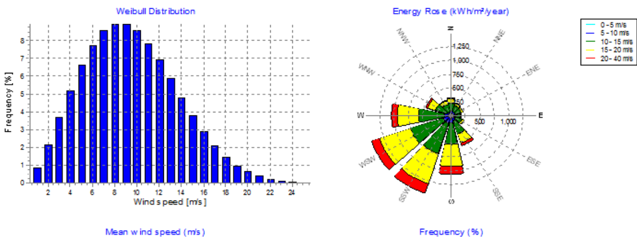
Figure 7.4.4: Weibull distribution and Energy rose (Source: WindPRO®)
