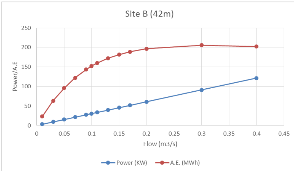
Figure 15.6.4 Seilebost-Flow, Power and Energy Relation Curve- Site B (42m) Source: Own Elaboration
