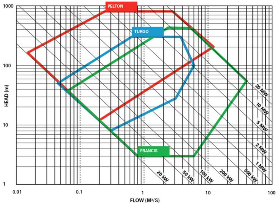
Figure 15.6.1 Turbine Selection Chart
