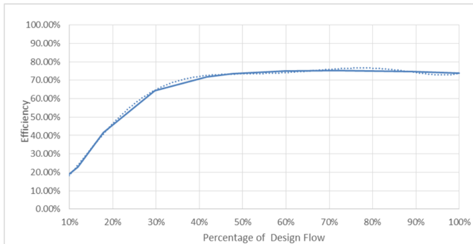
Figure 15.6.2 Overall Efficiency Curve (Penstock, Turbine and Generator)
