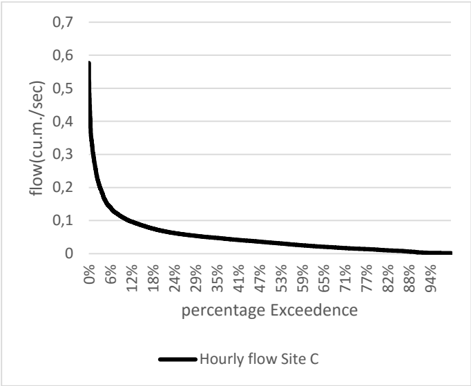
Figure 15.5.3 Flow Duration Curve Source: Own Elaboration
