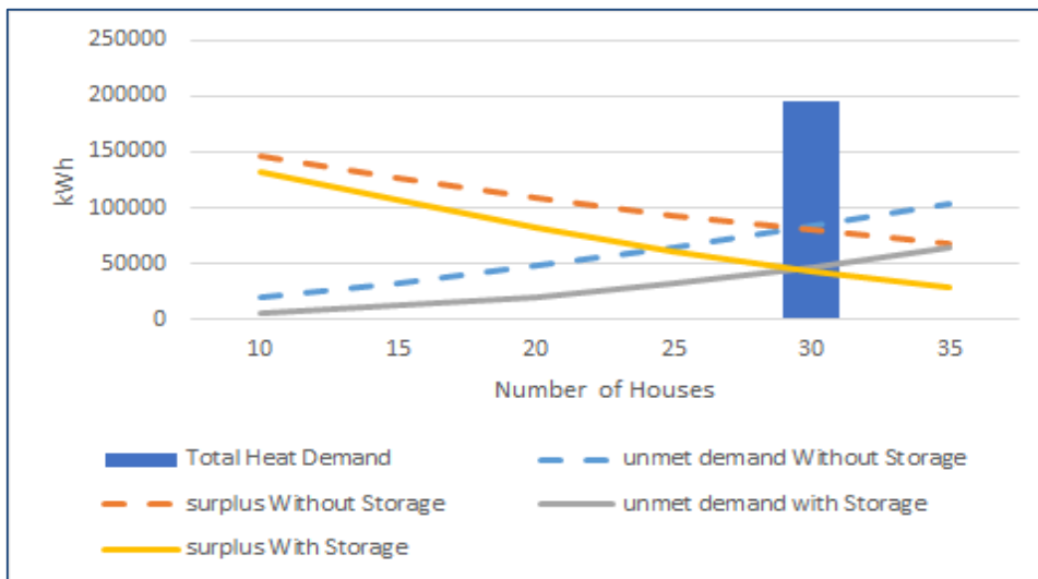
Figure 11.2.8: With Storage and Without Storage-Luskentyre (Intake Site B) Source: Own Elaboration
