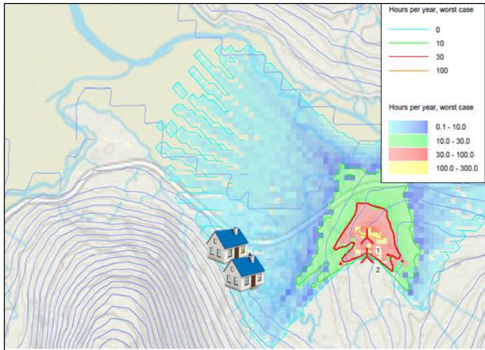
Figure 15.3.9 Glenn Dubhlinn Scenario III: Shadow map (Source: WindPRO®)
