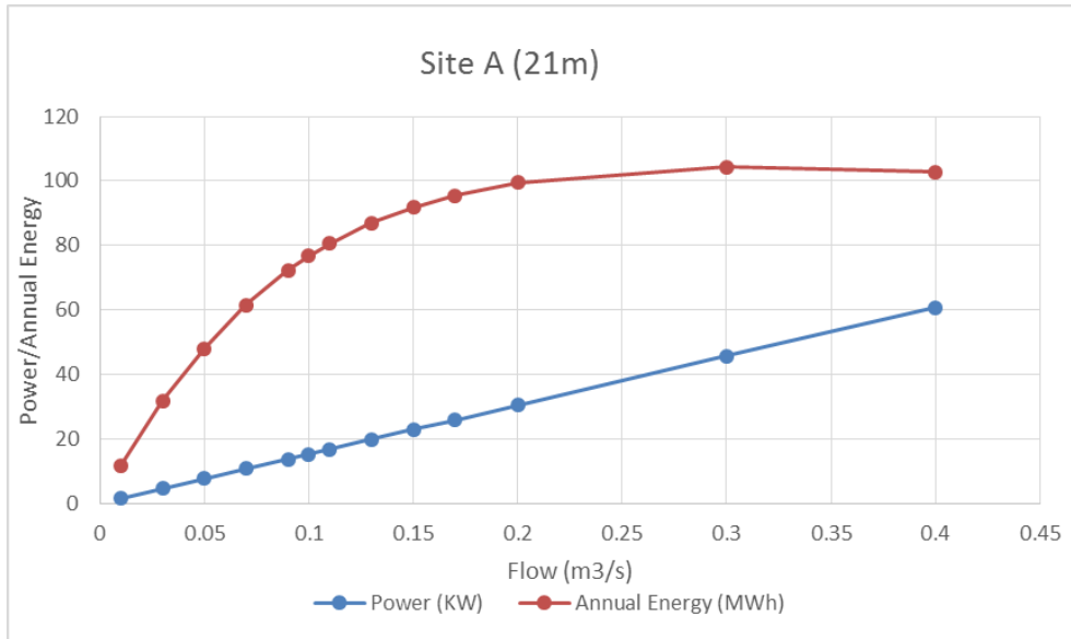
Figure 15.6.3: Seilebost-Flow, Power and Energy Relation Curve- Site A (21m) Source: Own Elaboration
